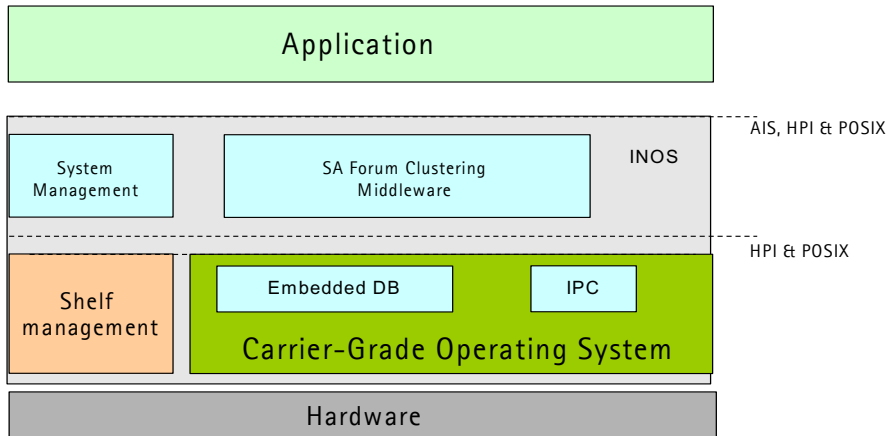
Fig. 2. Software architecture
