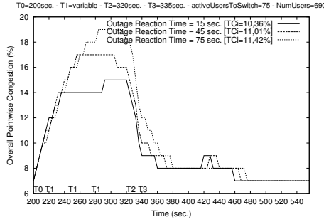
Fig. 10. Overall Congestion Perceived
