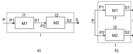
Fig. 2. Sequence and Choice Patterns
