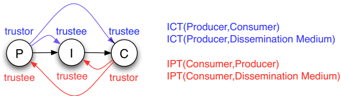
Fig. 3. Pairwise Trust Relationships within Information Lifecycle
