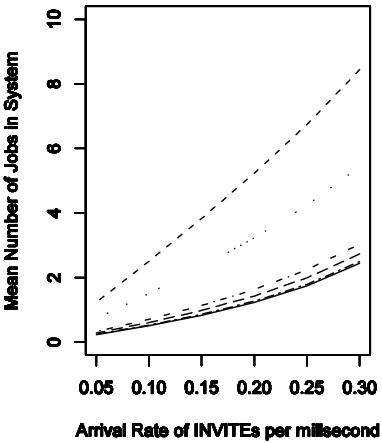
Fig. 5. Mean number of jobs under varying arrival rates
