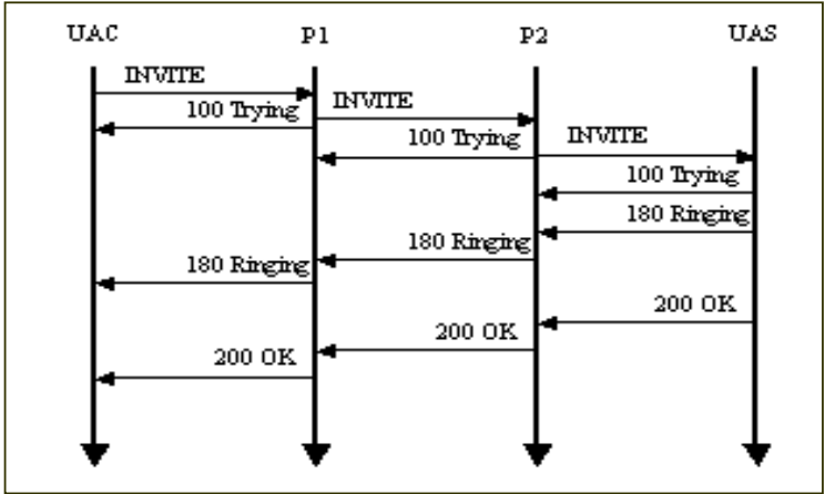
Fig. 1. SIP call establishment
