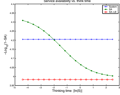
Fig. 9. SA vs. user think time
