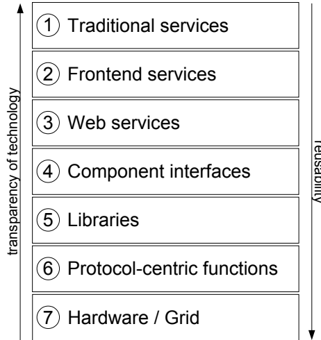
Fig. 2. Technology-oriented service layer model
