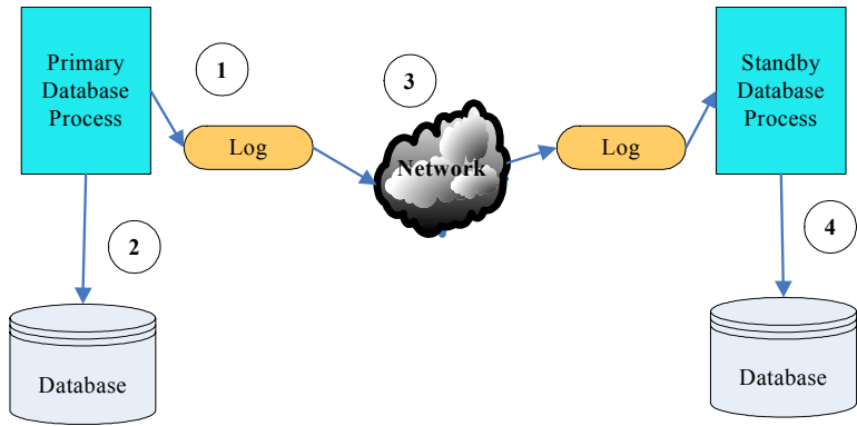
Fig. 5. Standby Database Operation
