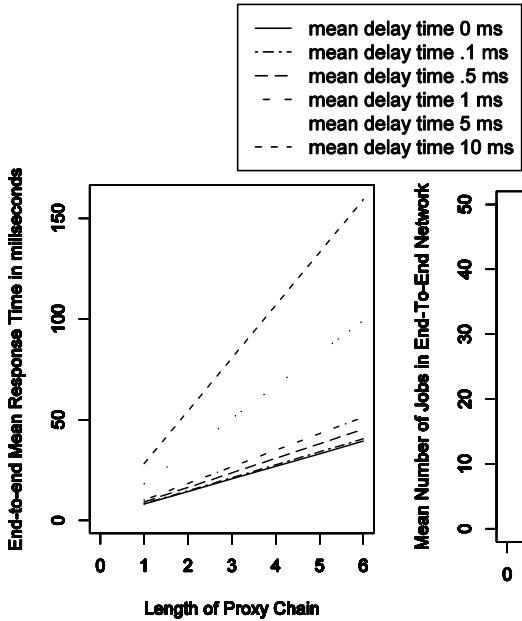
Fig. 11. End-to-end mean response time under varying length of proxy chains
