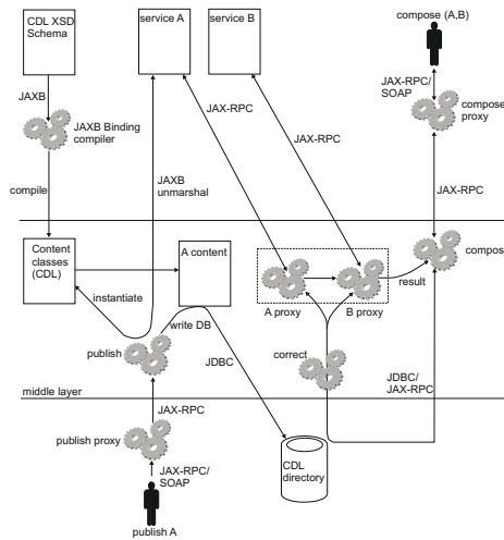
Fig. 5. JWSDP Runtime
