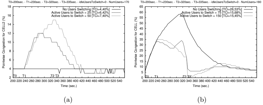
Fig. 7. (a) Congestion Perceived in CELL2 and (b) Congestion Perceived in CELL3
