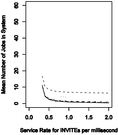
Fig. 7. Mean number of jobs under varying service rates
